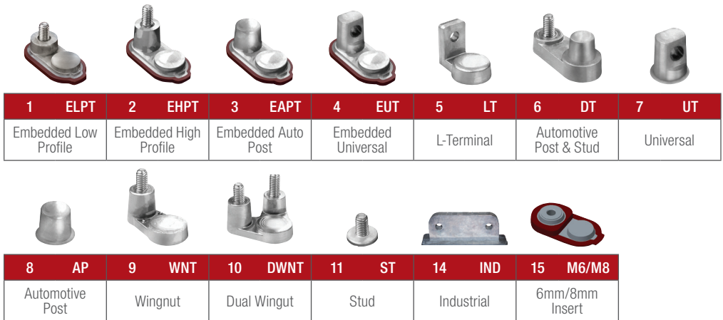
FIGURE 1 – TERMINAL TYPES
